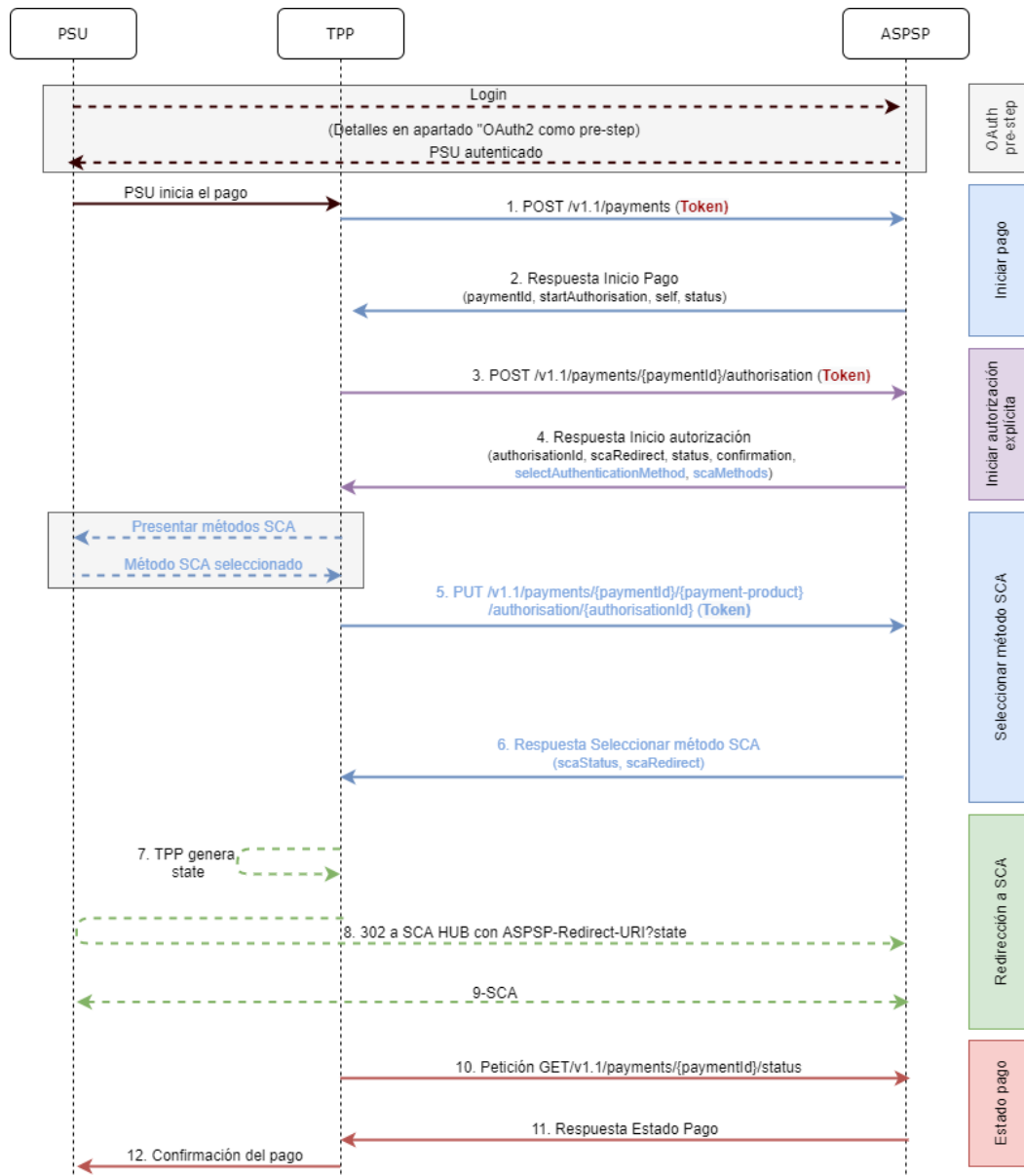
Figure 4: Start of payment with OAuth2 as pre-step and SCA flow by redirection and start of the explicit authorization process with / without selection of the SCA method
