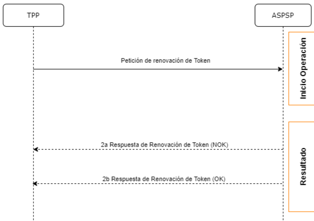
Figure 2: Access token renewal scenario
